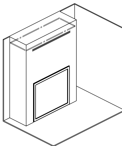
Figure 42: False Ceiling Iso View
