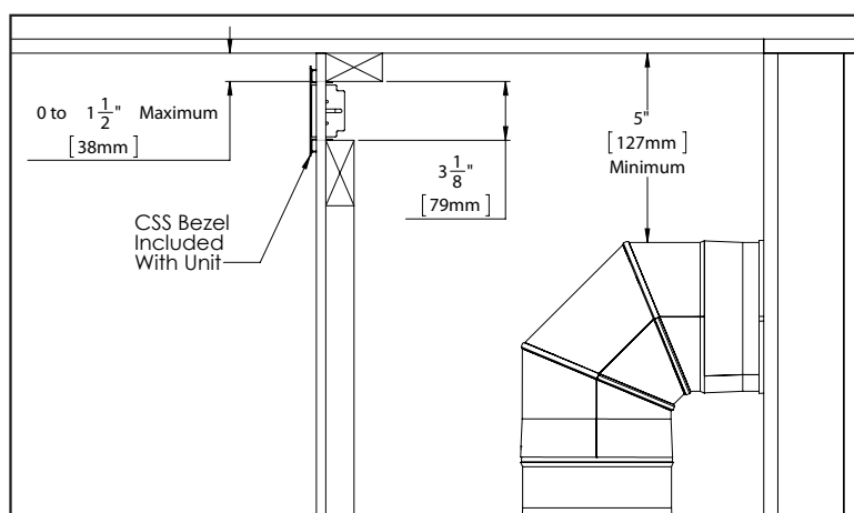
Figure 39: Option 3 Bezel
