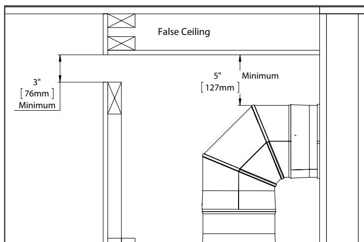
Figure 41: False Ceiling
