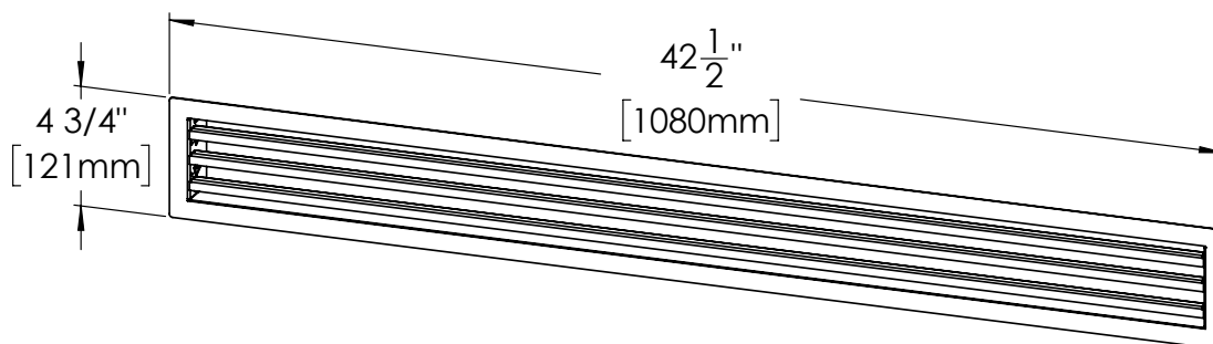
Figure 3: Front Bezel Iso View
