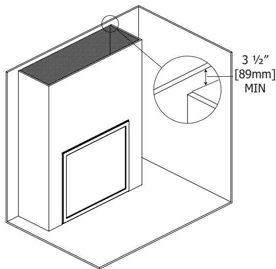
Figure 9: Open Chase Iso View
