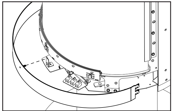
Figure 4: Skirt Removal
