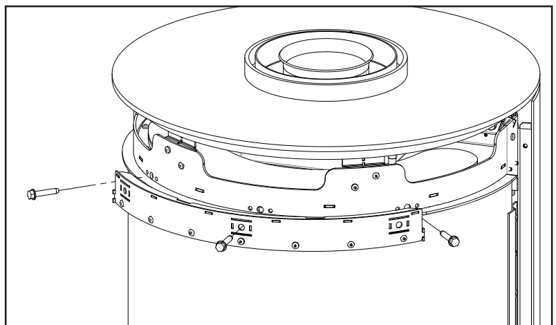
Figure 6: Glass Top/Bottom Clamps
