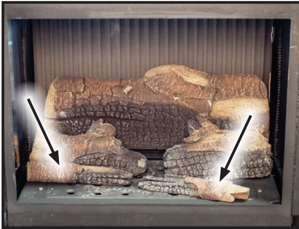
Figure 54. Log #2 & #3 Placement
