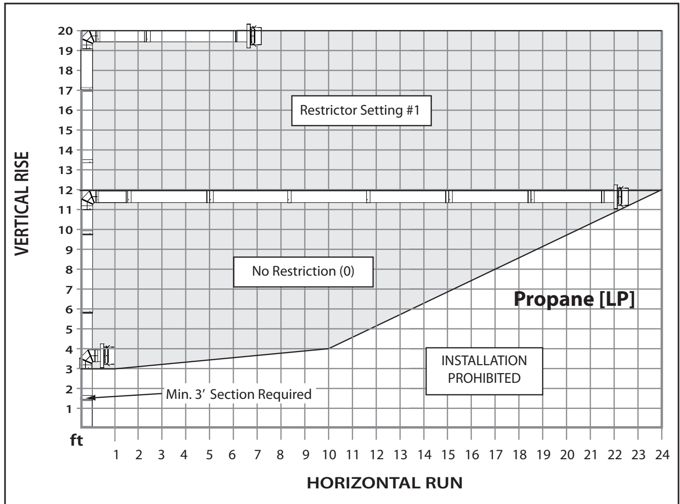
Figure 34: Horizontal Termination - 1 Elbow [LP]
