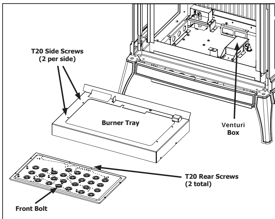
Figure 23. Burner Removal
