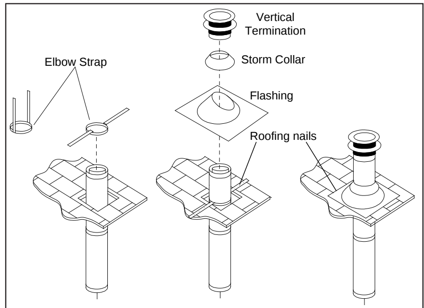
Figure 38. Vertical Vent Termination
