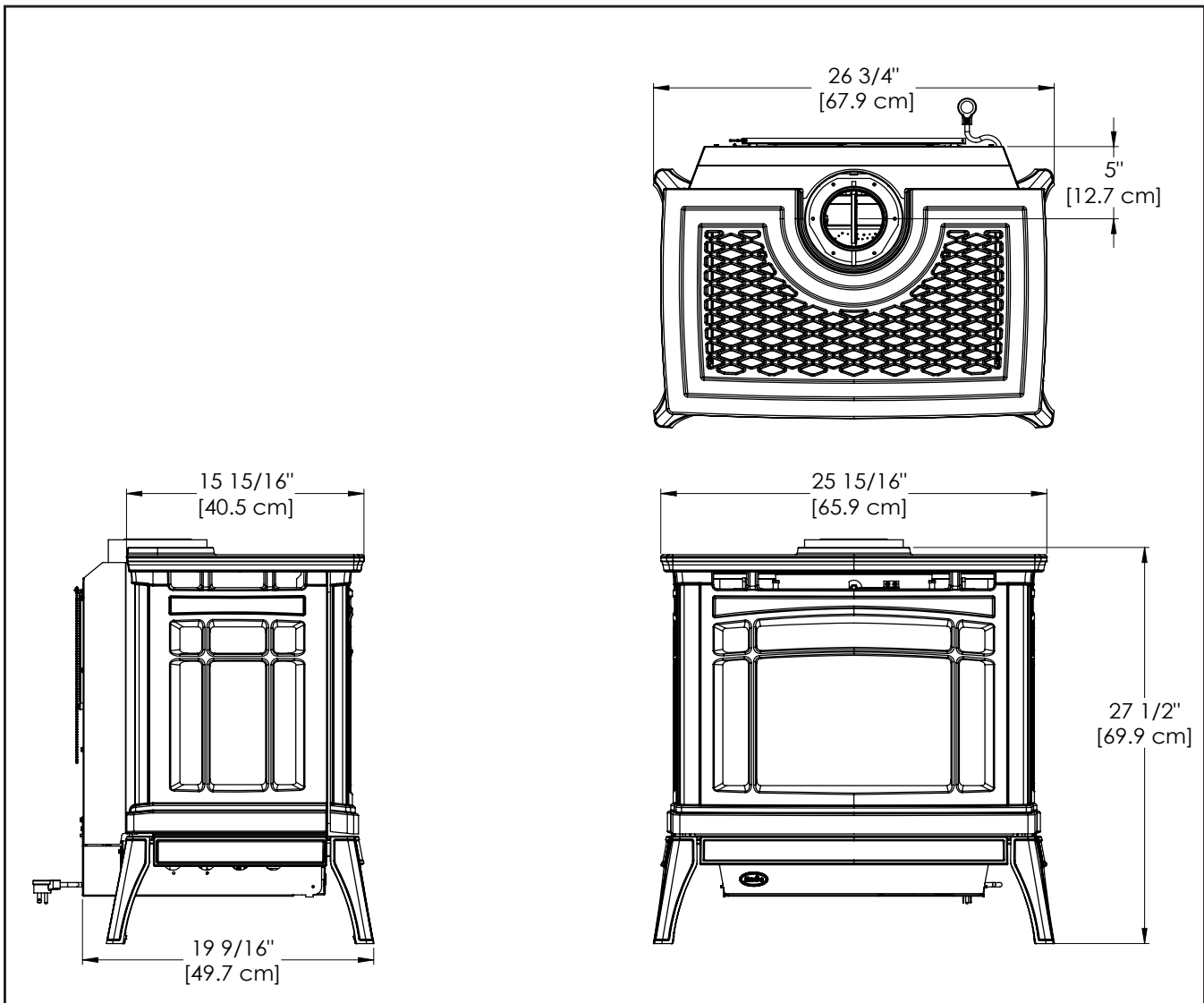
Figure 1. Westley Dimensions
