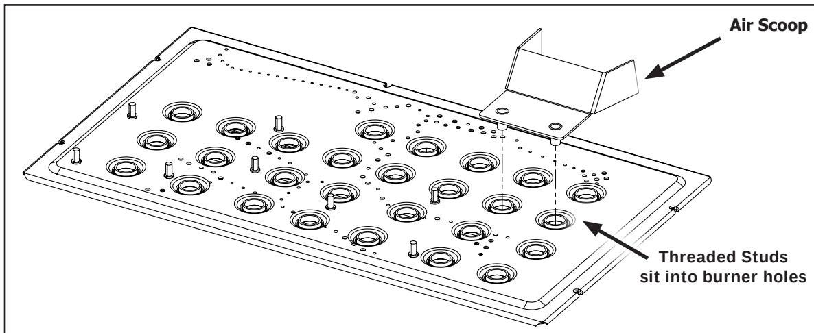
Figure 52. Air Scoop Installation
