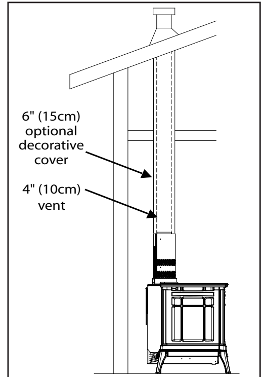
Figure 46: B-Vent Setup
