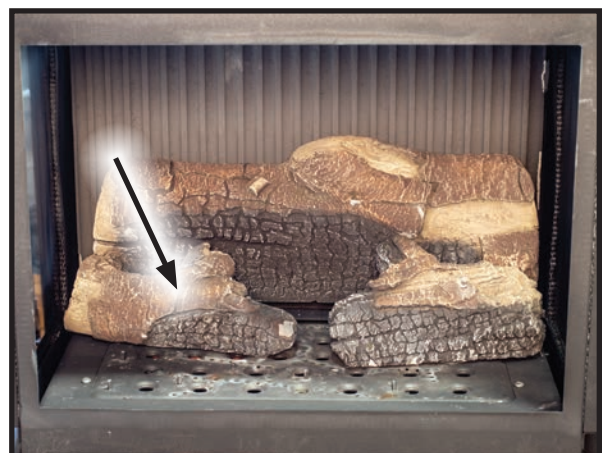
Figure 53. Log #5 & #6 Placement
