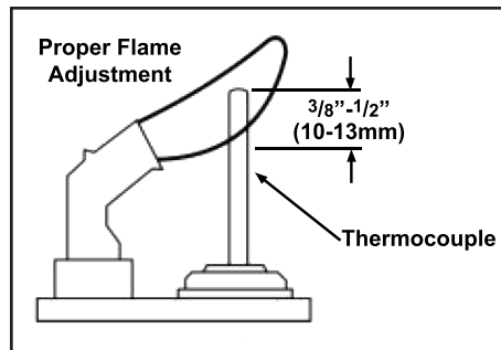
Figure 31: Proper Pilot Flame.
