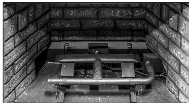
Figure 43: Remove the 6 screws highlighted in figure 42 using a Torx T-20 screwdriver and remove the air deflector
