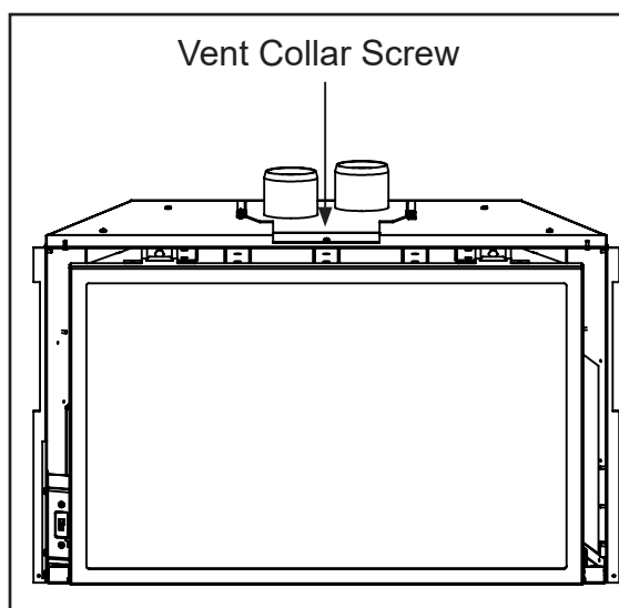
Figure 24: Vent Collar Plate Screw Location.
