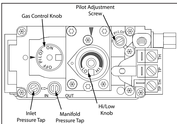
Figure 30: Valve Details.
