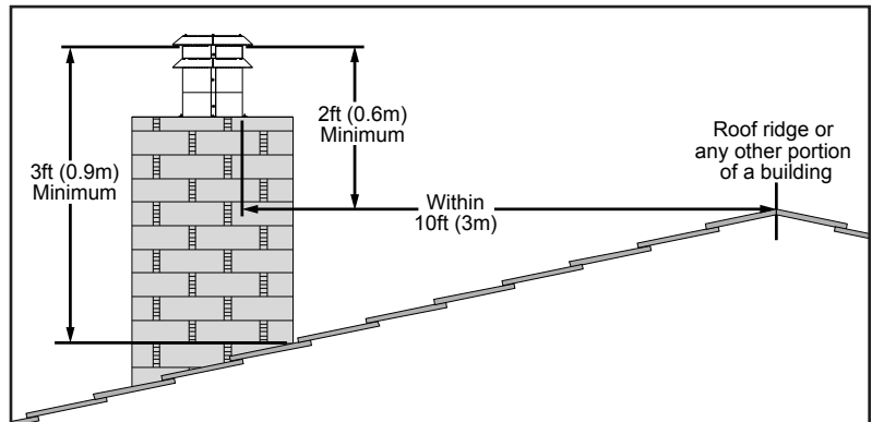
Figure 23: Roof Clearances.
