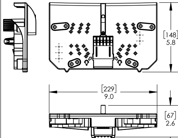
TOP PLATE OPZPT
