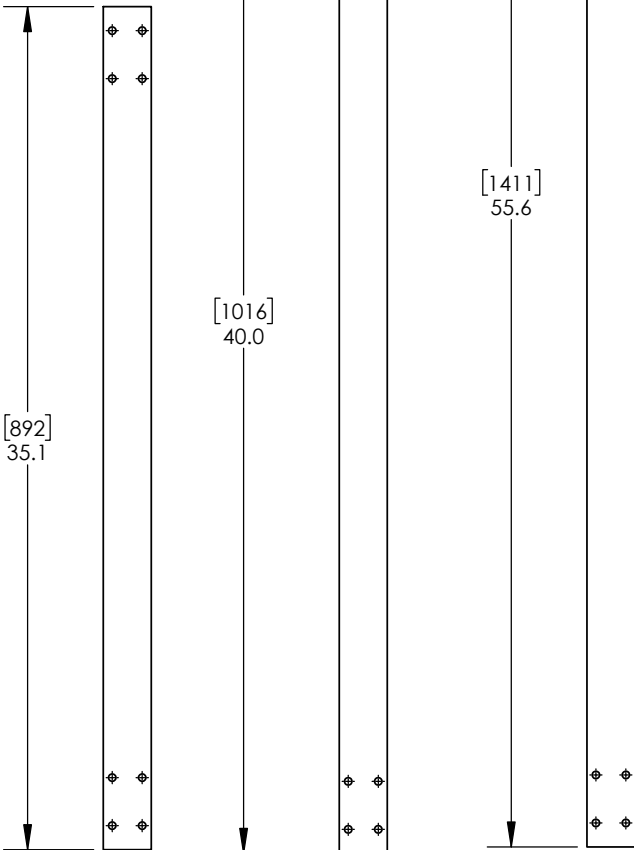
TIE STRAP 35" (46025007)
