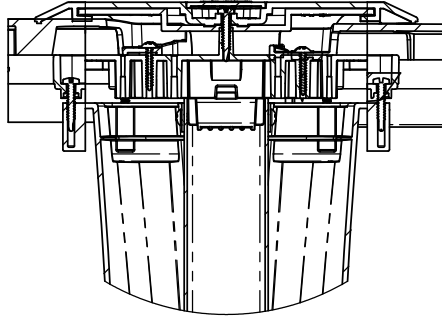
DETAIL L SCALE 1 : 5
