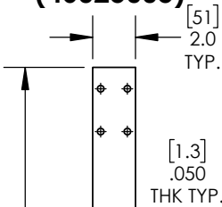
TIE STRAP 55" (46025005)
