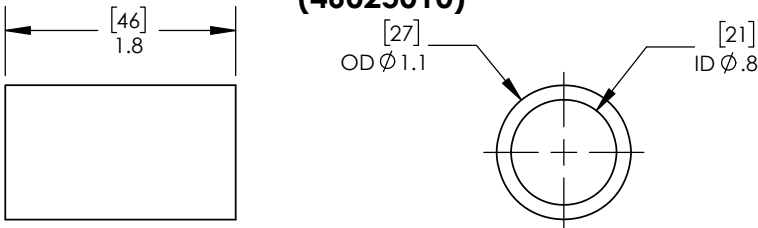
SLEEVE (46025010)
