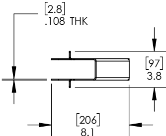
BUTTRESS POST (46025009)
