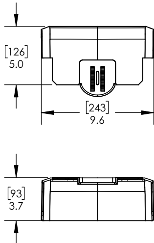
TOP LEDGE COVER REAR PDCB
