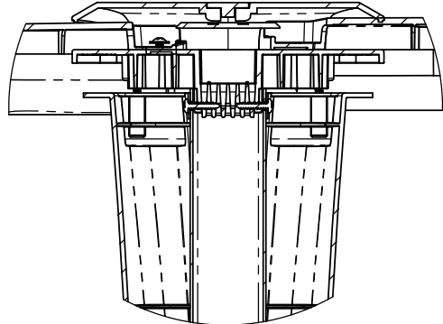
DETAIL I SCALE 1 : 5
