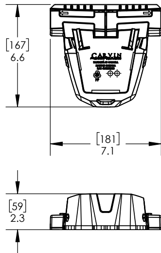
BOTTOM PLATE PDPB
