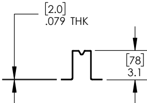
FOOT BEAM (46025008)
