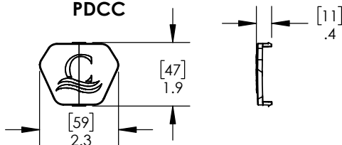
TOP LEDGE COVER CAP PDCC
