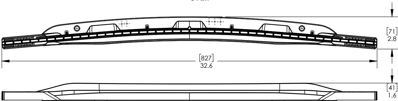
STRAIGHT RAIL TOP/BOTTOM OPZR
