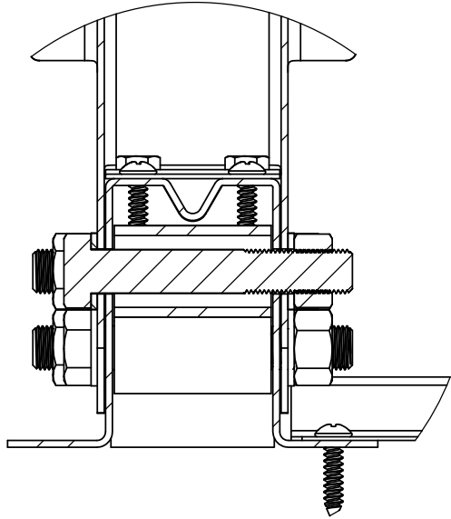
DETAIL D SCALE 1 : 2
