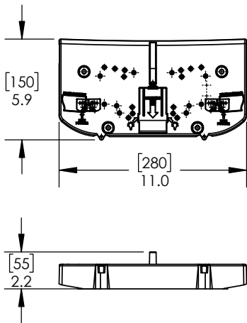
TOP PLATE PDPT
