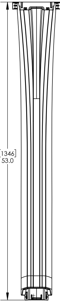
UPRIGHT PDU54
