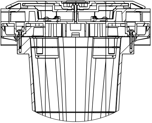
DETAIL N SCALE 1 : 4
